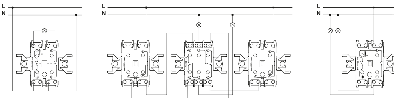
2-pole switch
